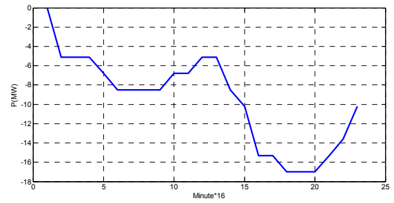
a) Load profile at node 3
