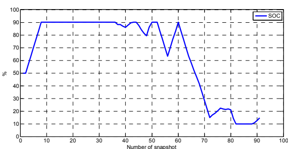
Fig.6. SOC of the battery at node 5
