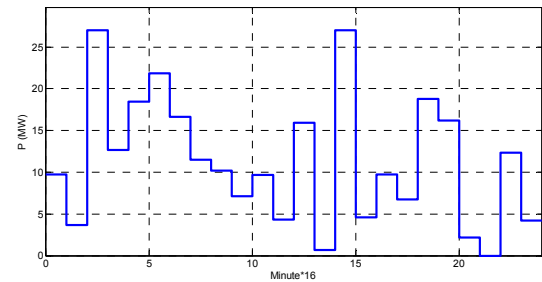
b) Power output profile at node 1
