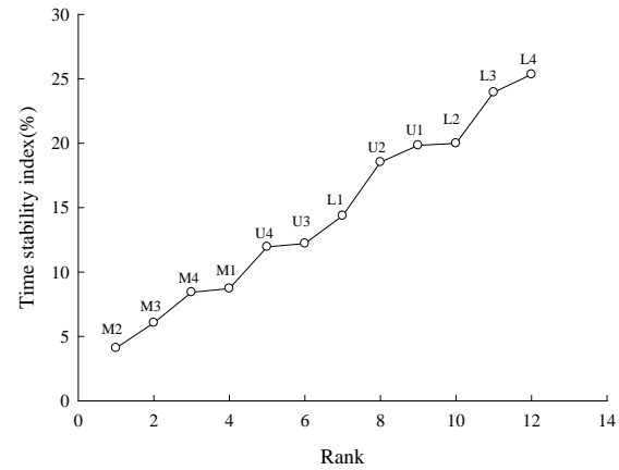
Fig. 3. Ranked temporal stability index of soil moisture
