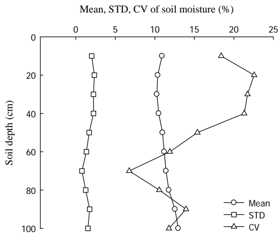
Fig.1. Mean value, standard deviation and coefficient of variation of soil water from May to September at different depths
