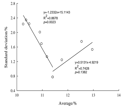
Fig.2. Relationship between average and standard deviation of soil water
