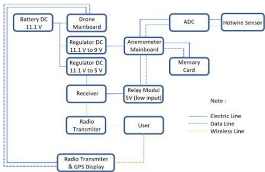
Fig. 4. Flow diagram of anemometer surveyor drone.
