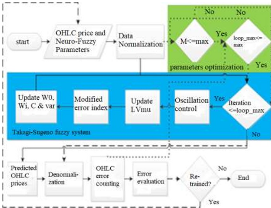
Fig. 2. Flowchart of the neuro-fuzzy working system.
