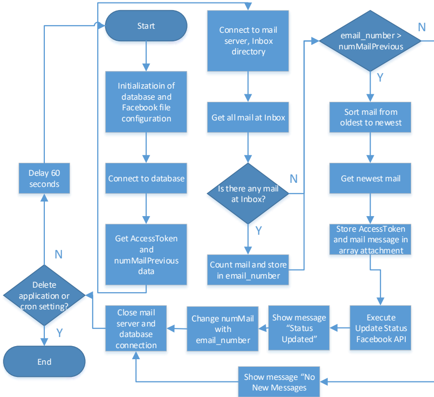
Fig. 3. Flowchart on the PagesUpStatus working application.
