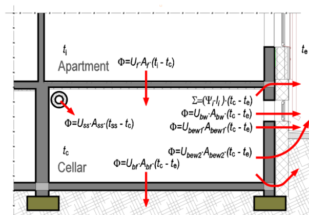
Fig 2 Heat balance of basement of an apartment building.
