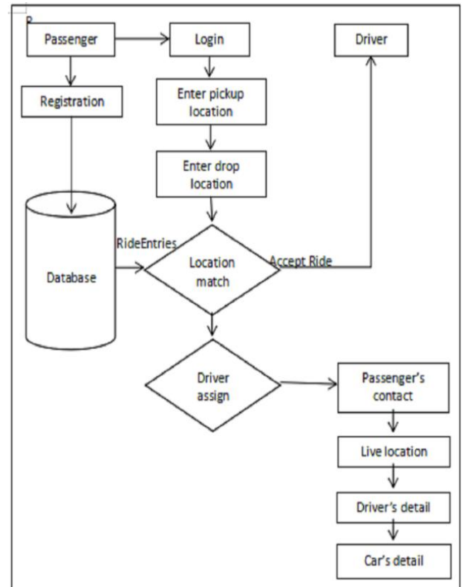
Fig.1. Flow diagram of carpooling system.
