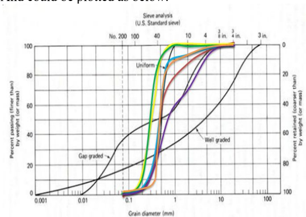
Fig. 5. Sieve Analysis
