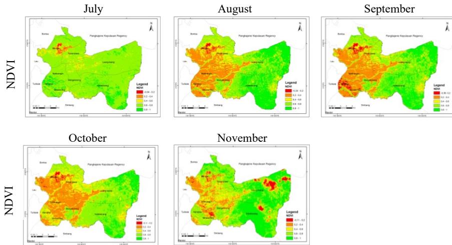
Fig. 5. Normalized Difference Vegetation Index (NDVI) from July – November 2015
