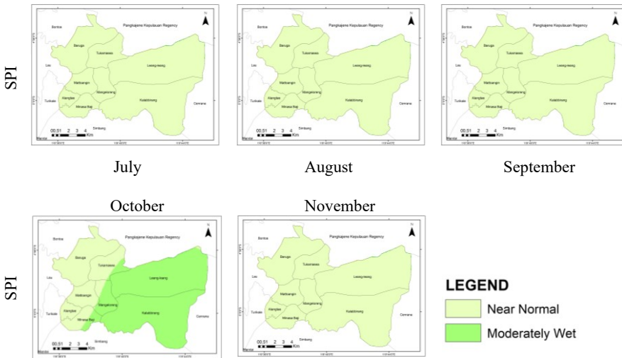
Fig. 2. Standard Precipitation Index (SPI) from July – November 2014
