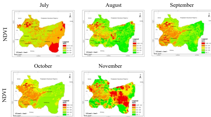
Fig. 4. Normalized Difference Vegetation Index (NDVI) from July – November 2014
