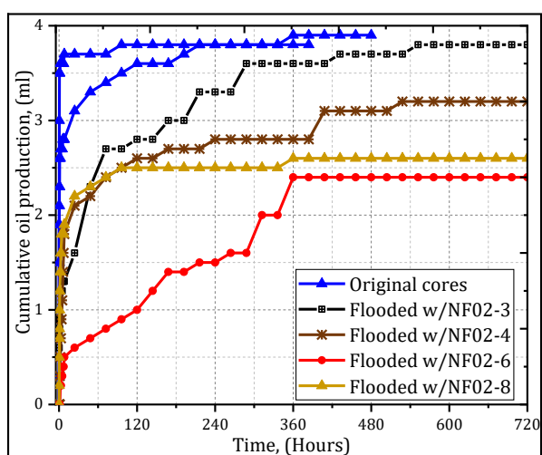
Fig. 5. Water spontaneous imbibition performed on cores flooded with nanofluids (at ambient conditions).
