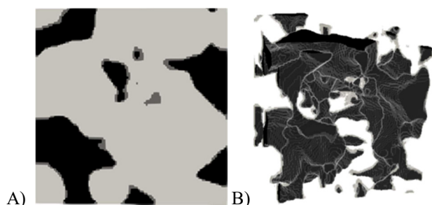
Figure 7: Cross-section (A) and 3D volume (B) images resulted from the comparison of segmentation methods: Hysteresis segmentation and AutoEncoder model. The black voxels are joint porosity of both segmentations and dark grey voxels are supplementary pore voxels in the Hysteresis segmentation.
