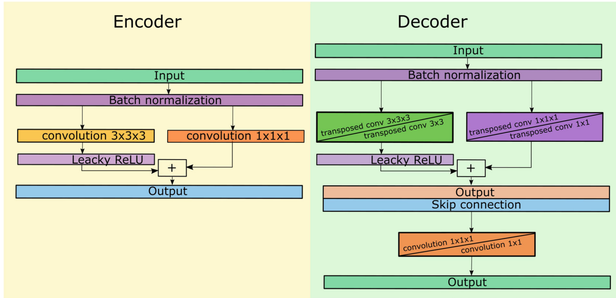
Figure 5: Single residual block of the encoder and decoder networks. After batch normalization, a first path leads through a (possibly strided) convolution or upsampling layer and a leaky ReLU. A second path either keeps the input or passes it through a strided (transposed) convolution in case it needs to be resampled. Both paths are added together to produce the final output. In the decoder block we skip connect the corresponding encoder features to the output of the decoder. The idea is that it is much easier for such blocks to learn the identity transformation, or perform only small modifications to the input [42], which helps the encoder-decoder paths to gradually add details.
