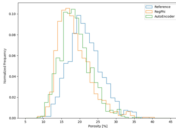
Figure 8: Porosity distribution computed by image analysis (reference), RegPhi and AutoEncoder models for Berea Sandstone sub-blocks.
