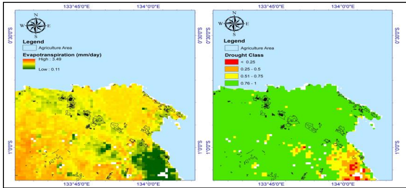
Fig. 5. Actual evapotranspiration and droughts on agriculture area on 17 March 2018
