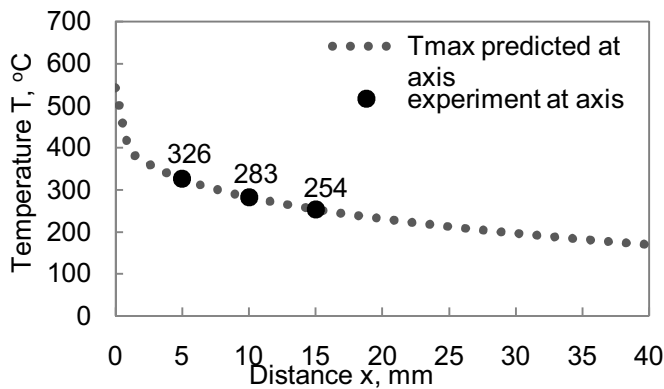
Fig. 6. The predicted of maximum temperature curves at axis on aluminium alloy side.
