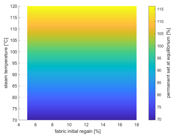
Fig. 13. Percentage of permanent set (equilibrium).
