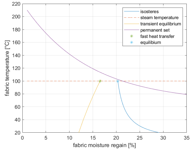
Fig. 7. Temperature rise predicted when the initial regain is low (yellow curve) and comparison with the equilibrium isosteres, enlightening the temperature the fabric should reach for being permanently set (purple curve).
