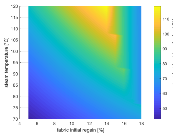
Fig. 14. Percentage of permanent set (heat transfer front).
