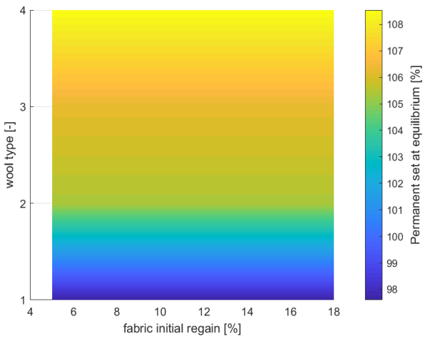
Fig. 10. Percentage of permanent set (equilibrium).
