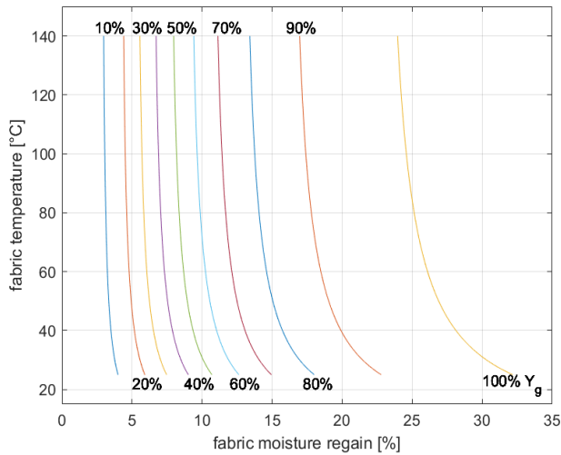
Fig. 6. Adsorption of moisture in wool at various relative humidities predicted by Equation 7.
