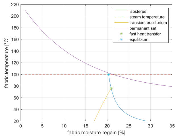
Fig. 8. Temperature rise predicted when the initial regain is high (yellow curve) and comparison with the equilibrium isosteres, enlightening the temperature the fabric should reach for being permanently set (purple curve).
