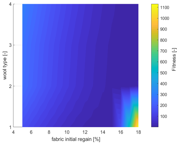
Fig. 9. Fitness function for four kind of fibers.
