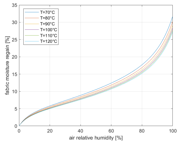
Fig. 5. Adsorption of moisture in wool at various temperatures predicted by Equation 7.
