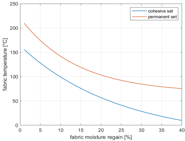
Fig. 3. Wool glass transition temperatures as a function of the moisture regain.
