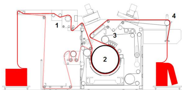
Fig. 1. Example of decatizing machine, composed of an entry unit (1), a steaming section (2), an aspirating section (3) followed by an exit one (4).
