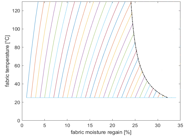
Fig. 4. Temperature rise predicted as steam condenses and absorbs into wool fabric during steaming, shown at different fabric regain.
