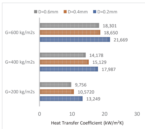
Fig. 4. Predicted heat transfer coefficients of condensation of R600a in microchannel for x_{in}=0.5 .
