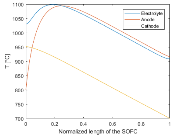
Fig. 7. Temperature distribution in the anode, electrolyte and cathode streams (0 indicates the anode inlet)
