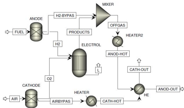
Fig. 2. Flowsheet of the model of SOFC in Aspen Plus®
