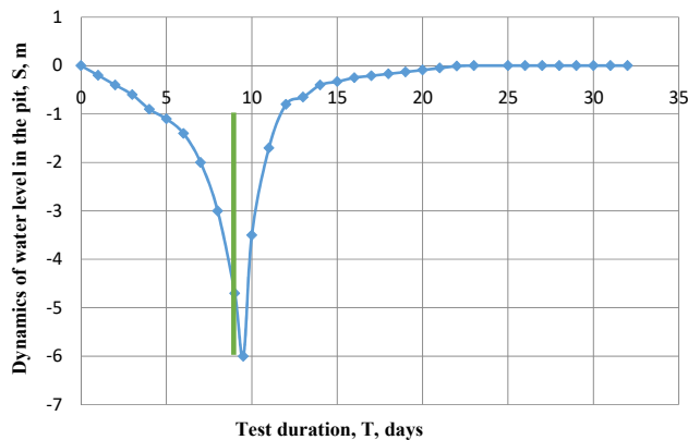
Fig. 1. Dynamics of lowering the water level and its subsequent restoration in a pit in dredging operations.
