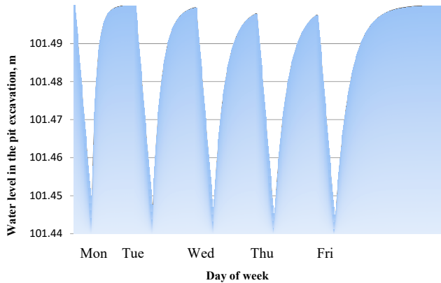
Fig. 2. Dynamics of water level fluctuations at the dredger operation Motronivskiy MPP pit during a working week.
