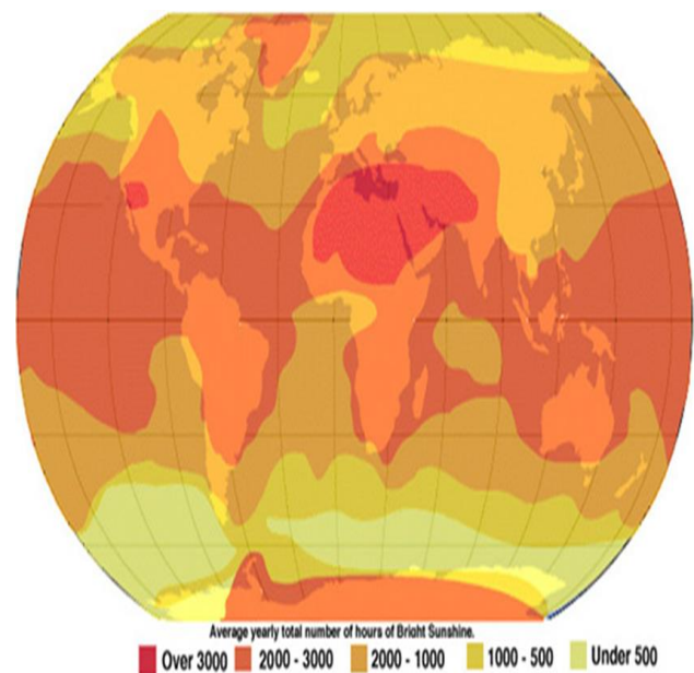
Fig. 3. Average yearly total numbers of hours of bright sunshine
