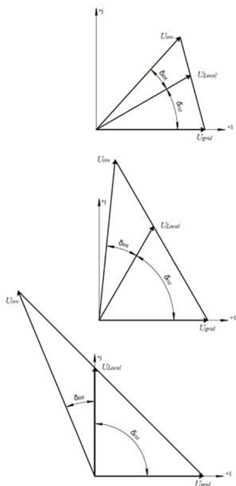
Fig. 9. Vector voltages diagram at different values of the angle \delta
