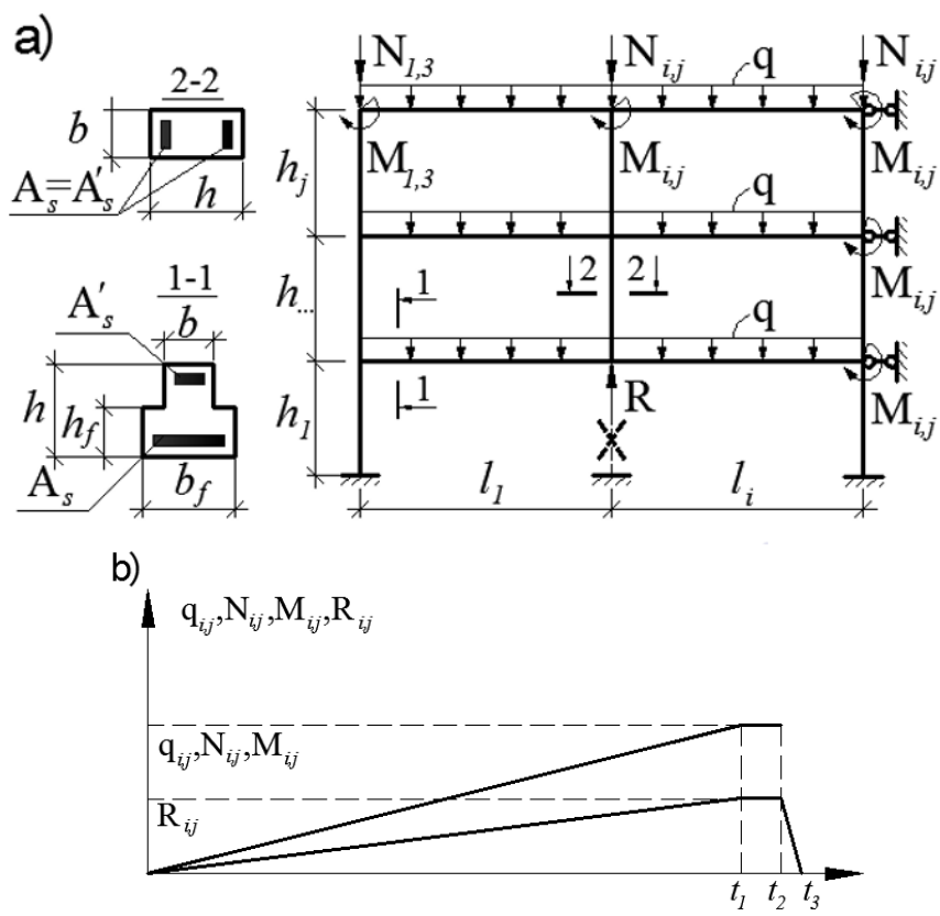
Fig. 3. A design scheme of a fragment of the substructure of the building frame (a) and scheme of its loading (b)
