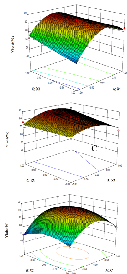
Fig. 2. The 3-D plots of variables (X1: temperature; X2: ultrasonic power; X3: time) on the yield of inulin.
