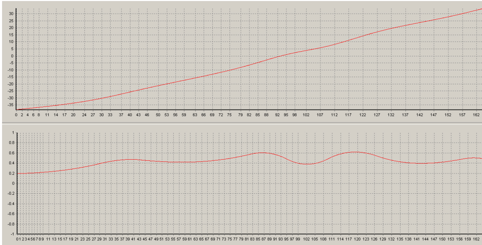
Fig. 3. Pitch angle (upper figure) and pitch angular velocity (lower figure) during imagery using TDI mode (spline approximation of the survey object).
