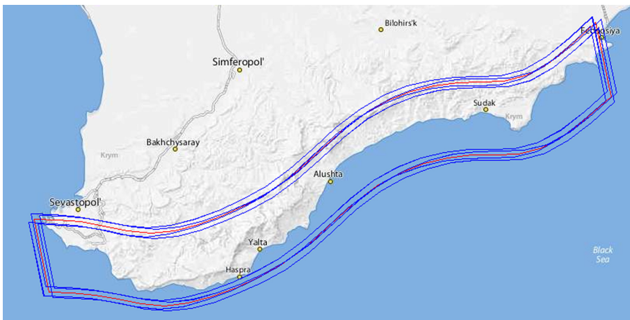
Fig. 2. Modeling satellite imagery with the account of the maximum satellite attitude errors \pm 0.1^\circ in roll, pitch and yaw.
