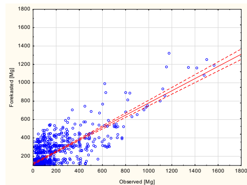
Fig. 3. The predicted versus the observed values of material released in an outburst in the “Piaś” field of the former “Nowa Ruda” mine for the training set.
