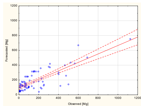
Fig. 4. The predicted versus the observed values of material released in an outburst in the “Piaś” field of the former “Nowa Ruda” mine for the validation set.
