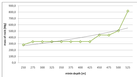
Fig. 5. Mass of rocks released in hypothetical geological and mining conditions, as a function of mining depth.
