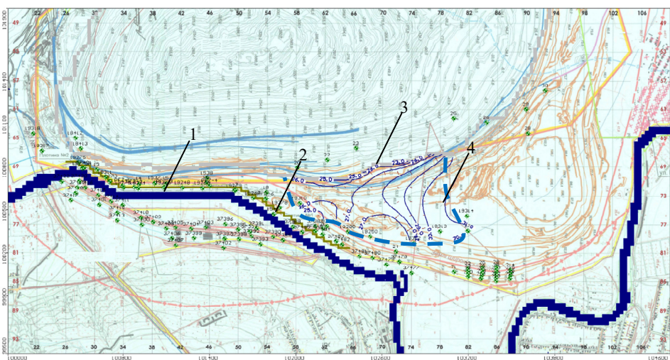
Fig. 5. MODFLOW-simulated groundwater heads at the baseline of №3 rock-disposal dump as of April-May 2015 – inverse problem solution, transient flow regime, m: 1 – current position of the Inhulets River; 2 – seepage cutoff wall; 3 – groundwater flow direction; 4 – technogenic aquifer.
