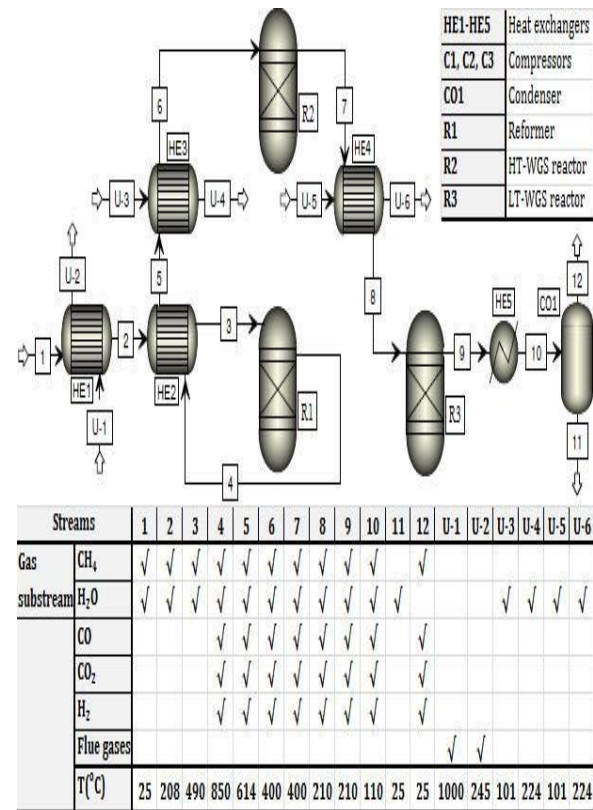
Figure 1. Steam Methane Reforming Process Working Principle [38]
