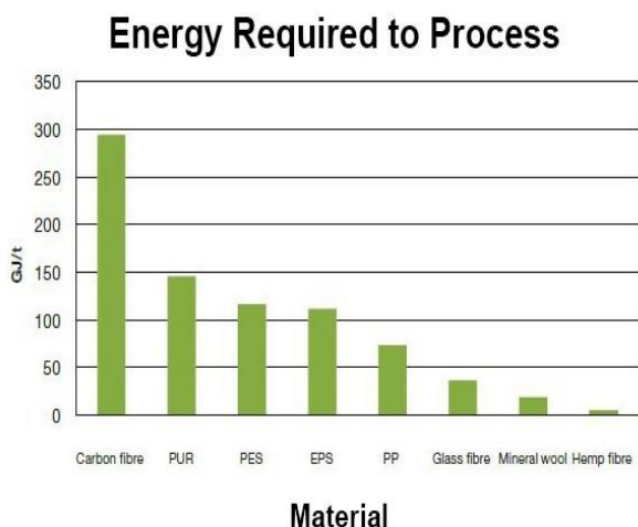
Figure 9. Energy required for the production of different type of plastics.
