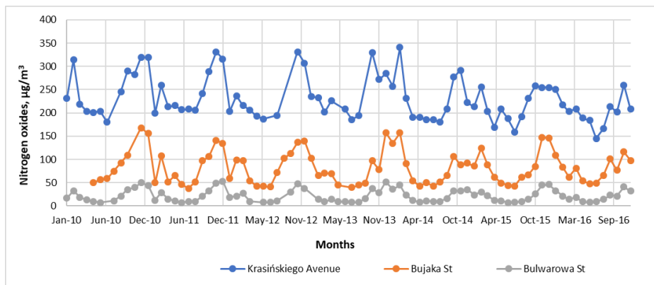
Fig. 3. NO x content in the air in Krakow in 2010–2016. Source: own work based on [12]
