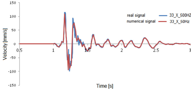
Fig. 4. Run of the horizontal component of the excitation, taking account of the frequency of sampling in the numerical program [11]
