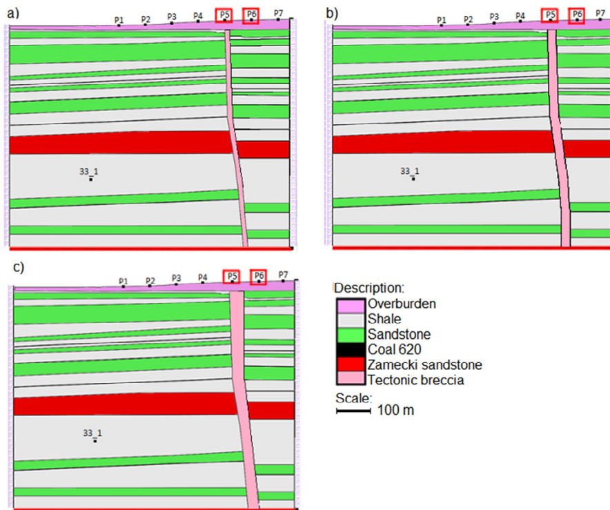
Fig. 3. Area covered by the numerical analysis. Location of points (P1 to P7) on the area surface, together with point 33_1 of the input excitation task, a) - fault zone of 15 m in width, b) – actual width of the fault zone 30 m, c) fault zone of 45 m
