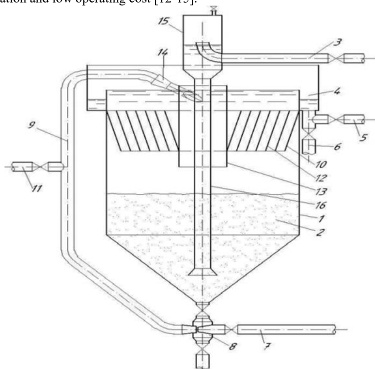
Fig. 1. Reactor-clarifier
