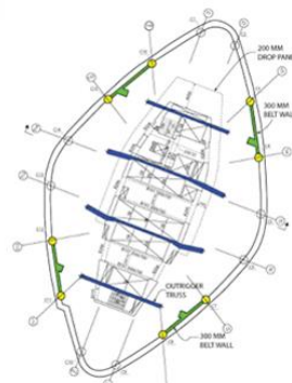
Fig 9: Outrigger
