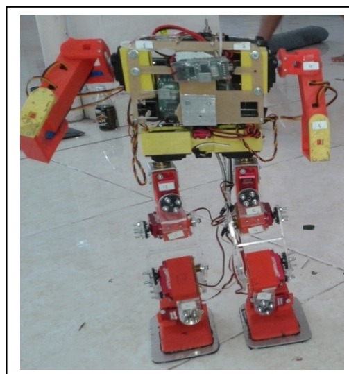
Fig. 3. Physical form Mechanical Robot
