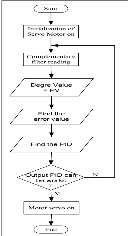
Fig. 4. Flowchart Robot
