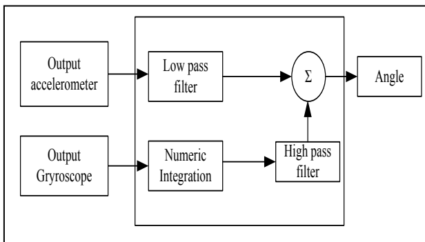
Fig. 5. Diagramm Block Complementary Filter
