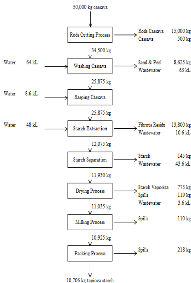
Fig. 1. Flowsheet diagram of tapioca starch production process.
