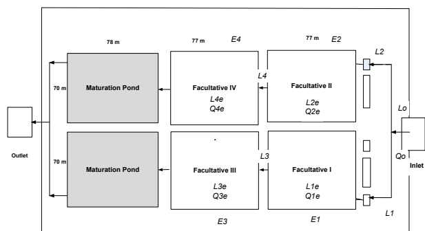
Fig. 1. Wastewater Treatment Scheme in Facultative Pond
