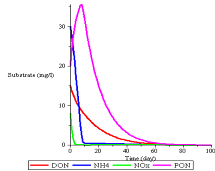
Fig. 3. Behavior of Substrate Concentration
