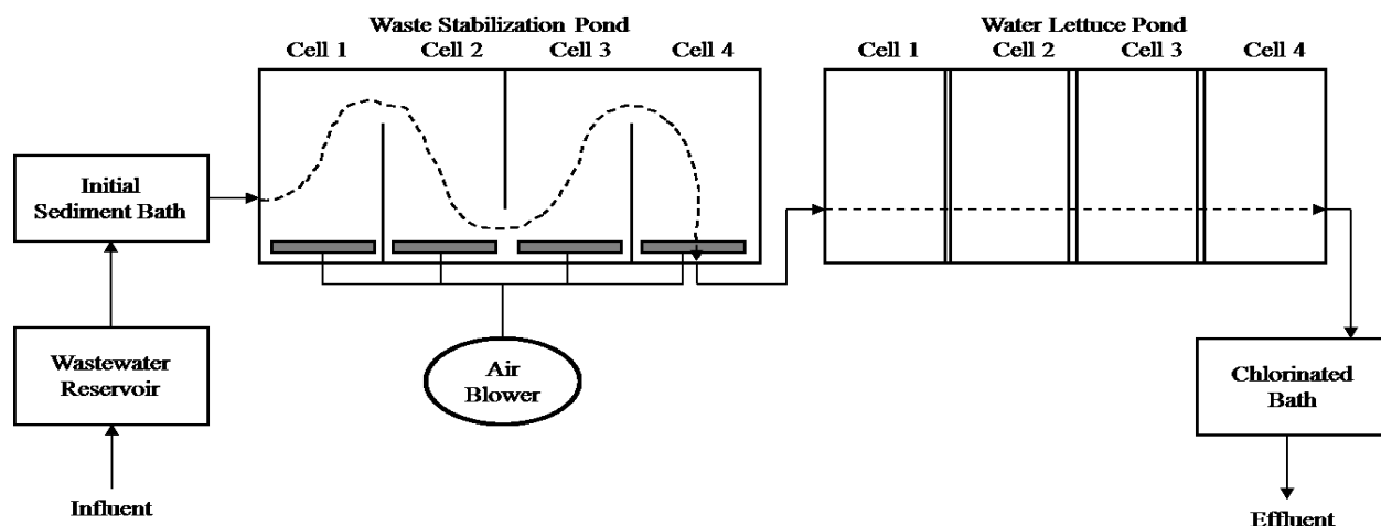
Fig. 1. Pilot System Layout
