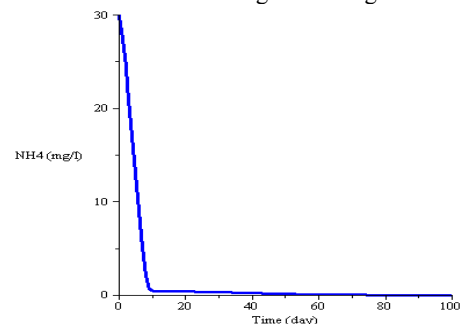
Fig. 6. Behavior of Ammonium Concentration
