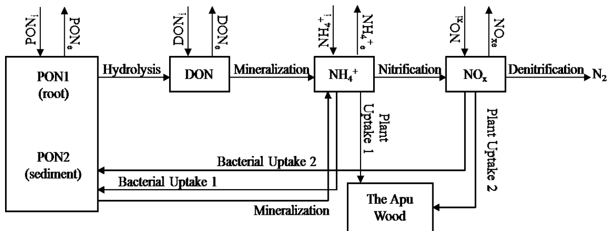
Fig. 2. Conceptual Model of Nitrogen Transformation in the Water Lettuce Pond
