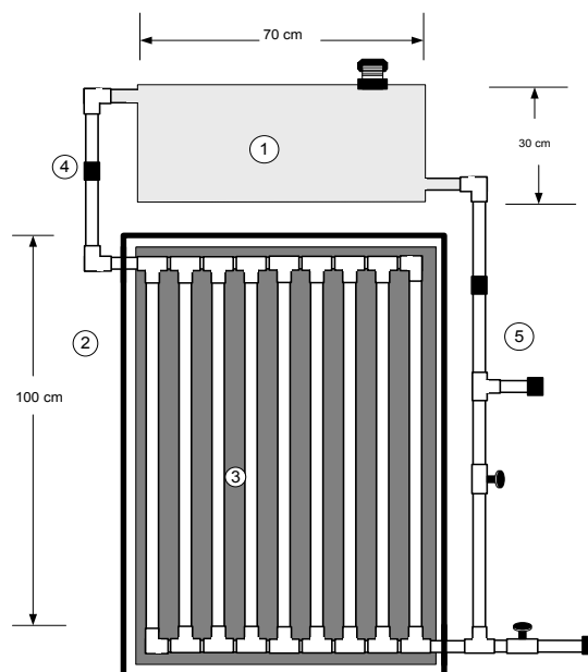
Fig.1. Design of Solar Water Heating System
