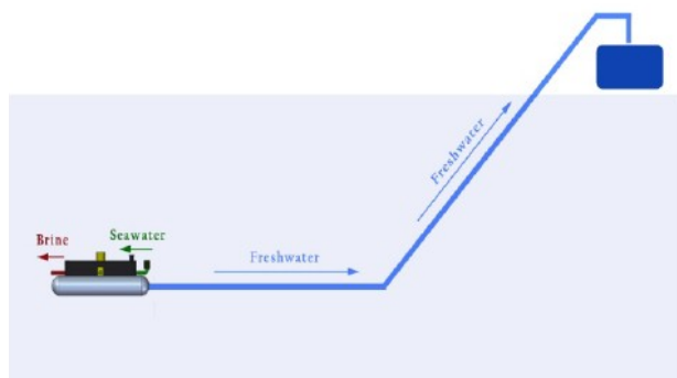
Fig. 2. Deep sea reverse Osmosis scheme[19]
