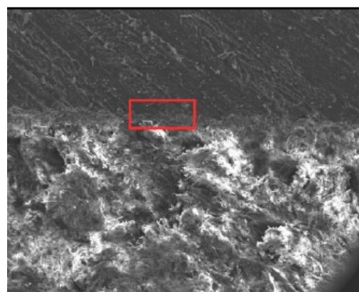
(a) SEM & EDS test of interface between wood and resin-ramie before field test
