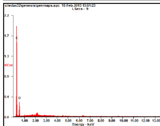
(a) SEM & EDS test of interface between wood and resin-ramie before field test
