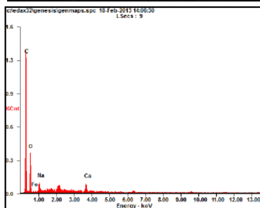
(b) SEM & EDS test of interface between wood and resin-ramie after 5.5 months field test
