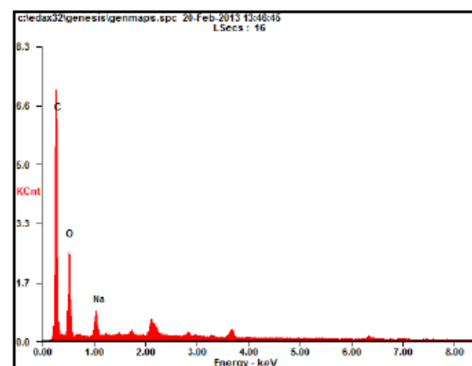
(b) SEM & EDS test of resin-ramie part after 5.5 months field test
