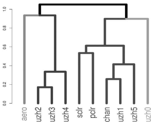
Fig. 1. Ward clustering of a matrix of Kulczynski distances among stations. Data were Hellinger transformed. Stations: aéro — aeration tank, chan — derivation channel, pclr — primary clarifier, sclr — secondary clarifier, uzh0 — river 50 m upstream the treated wastewater discharge, uzh1 — river at the discharge site, uzh2, uzh3, uzh4, uzh5 — river 50, 100, 250 and 300m.
