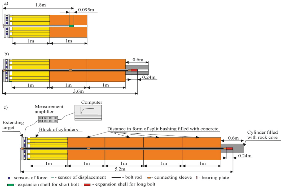
Fig. 2. Arrangement of sensors and elements of rock bolt support on the laboratory test facility; a) rock bolt support with a length 1.8 m, b) rock bolt support with a length 3.6 m, c) rock bolt support with a length 5.2 m.
