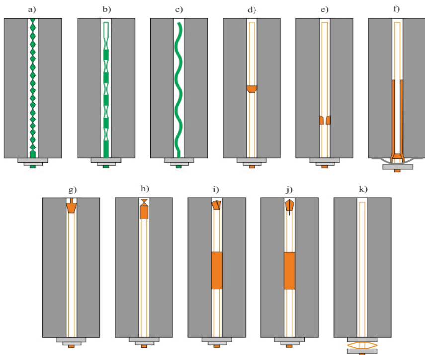
Fig. 1. Simplified mechanisms for absorbing of energy by rock bolts; a) “CTw”, b) “D”, c) Durabar”, d) “Roofex”, e) “Garford”, f) “He”, g) “Modified Cone bolt”, h) “Dynatork” i) “DAP”, j) “NMX”, k) “Deformable component”.
