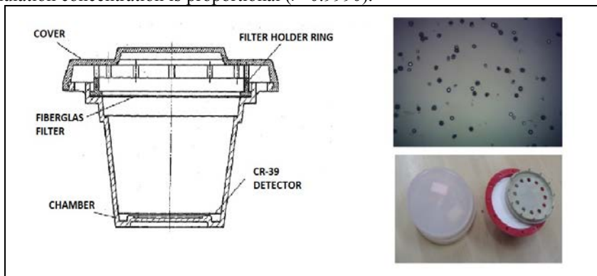
Fig. 1 Karlsruhe-type passive time integrating radon detector
