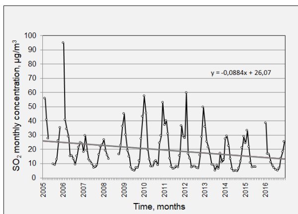
Fig. 5. The course of monthly average concentrations of SO 2 at the Zabrze station in the period 2005-2016 with adjusted linear trend.
