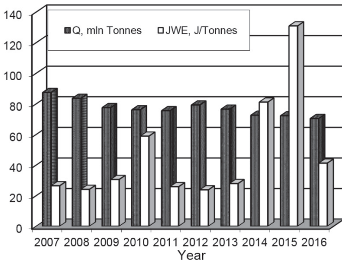
Fig. 1. Unitary Energy Expenditure compared to coal extraction in hard coal mines of GZW in 2007-2016.
