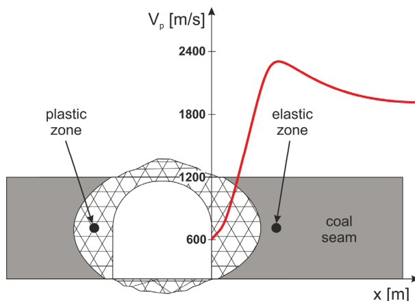
Fig. 2. An example of changes in P-wave velocity in the side-wall of the excavation [18].
