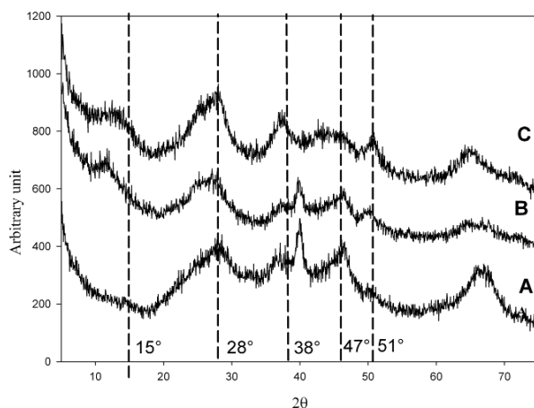
Fig. 1. XRD patterns of Pt doped oxides: A – 1% Pt/BAI 0.25, B – 1% Pt/BAI 0.5, C – 1% Pt/BAI 1.0.
