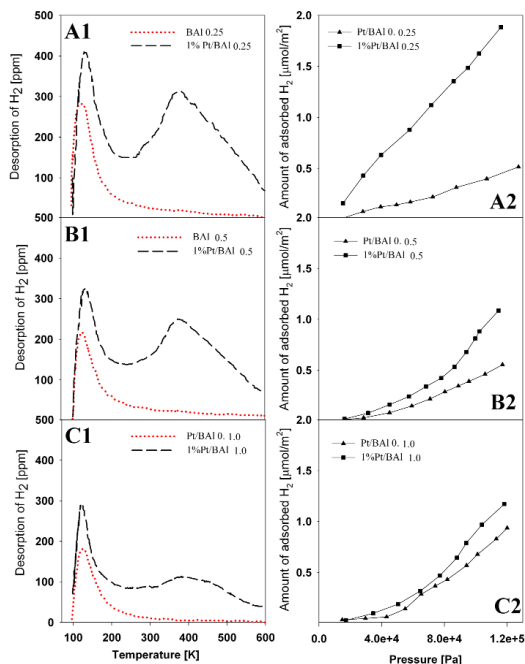
Fig. 4. Hydrogen adsorption isotherms: A. TPD method: A1 – 1% Pt/BAI 0.25, B1 – 1% Pt/BAI 0.5, C1 – 1% Pt/BAI 1.0. B. Volumetric method: A2 – 1% Pt/BAI 0.25, B2 – 1% Pt/BAI 0.5, C2 – 1% Pt/BAI 1.0.
