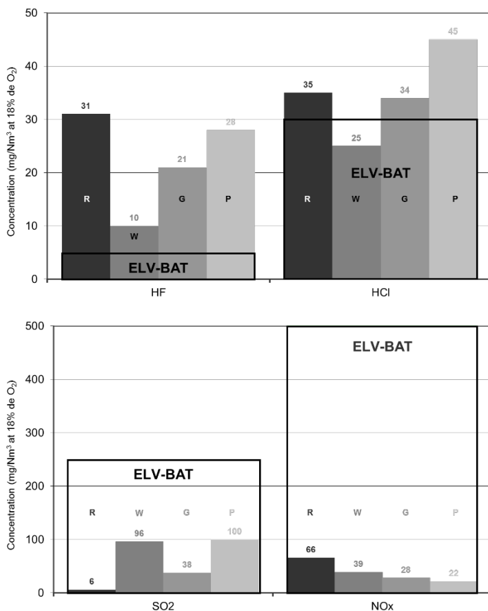
Fig. 1. Median acid pollutant concentrations for earthenware (red (R) and white (W)-firing body), glazed stoneware tile (G) and porcelain stoneware tile (P) in the firing stage.
