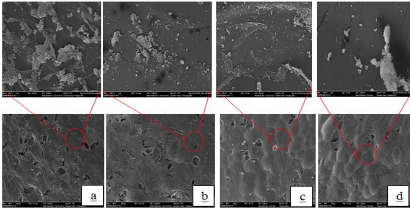
Fig. 6. SEM images of hybrid coatings of the different photo-initiators for UV curing (a: PS-S2, b: PS-S3, c:PS-S4, d: PS-S5 and top: 5000 mag., bottom: 100 mag.).
