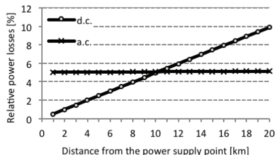
Fig. 3. Relative power losses for the power supply of one station with the capacity of 150 kW, depending on the distance from the power supply point.
