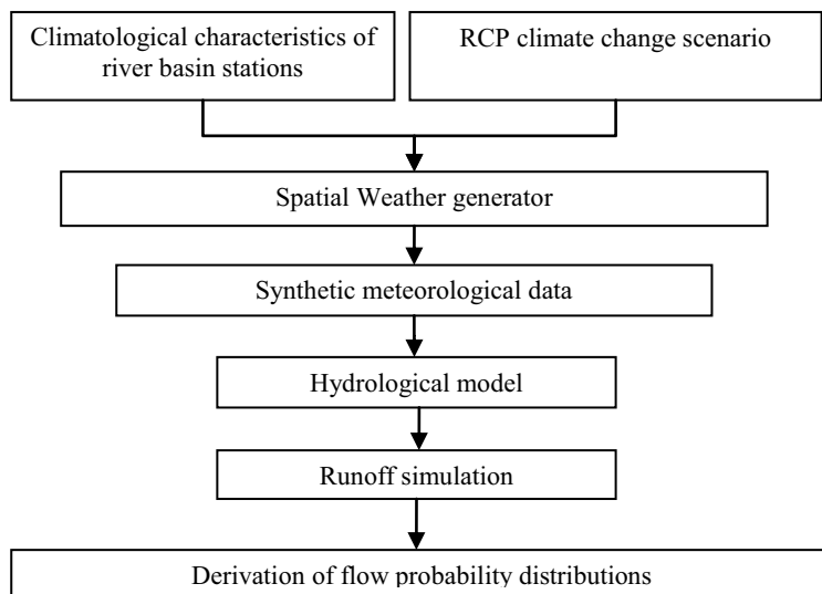
Fig. 1. Diagram of river flow simulation for future climate using synthetic meteorological data and climate change scenario.
