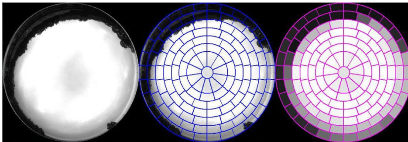
Fig. 4. Luminance distribution in Białystok 11-th of July a) HDR sky image, b) with Tregenza mesh, c) with mesh and averaged luminance.
