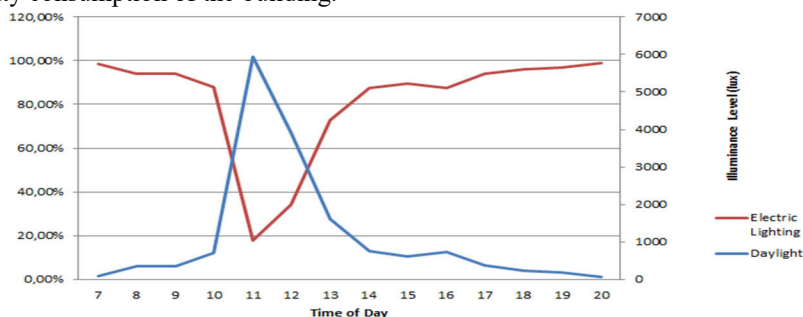
Fig. 1. The result of daylight automatic control is energy savings for 23 July 2016 (Clear sky).
