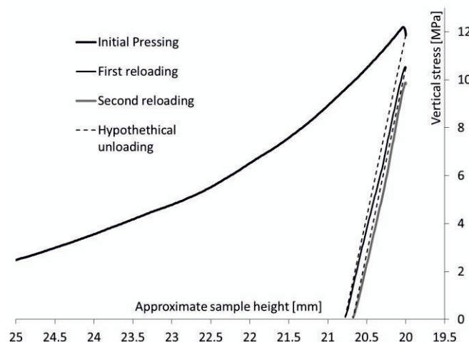
Figure 3. Vertical stress and displacement during sample pressings. No unloading data is available – the unloading paths are hypothetical. The vertical stress value is based on the press force readout. The target sample height was 20 mm. Pressing resulted in sample of Sr=0.59 and dry density 1.56 g/cm 3
