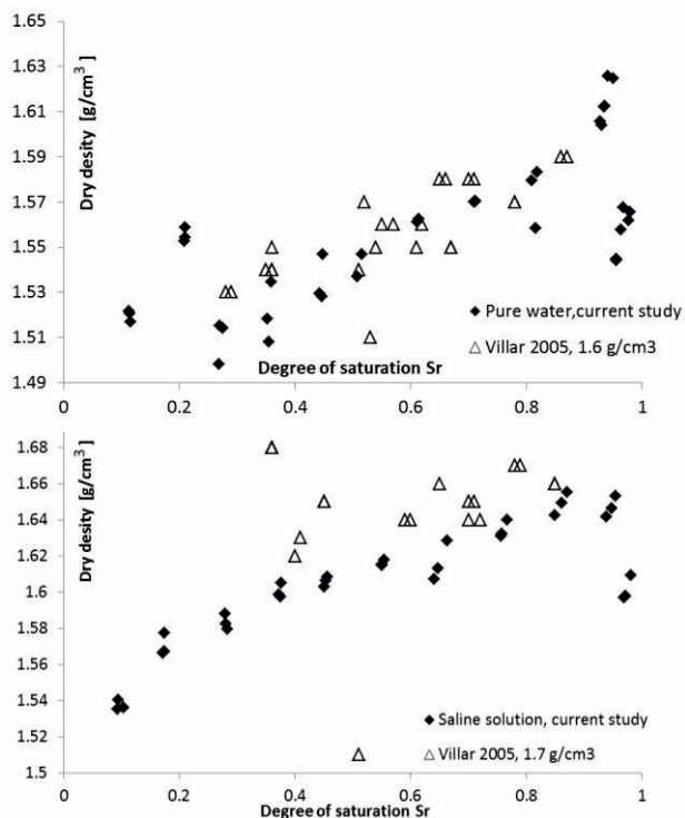
Figure 4. Variation of dry density in the current study and in [1]. For comparison, data for samples with target dry density of 1.6 and 1.7 g/cm 3 are shown [1].
