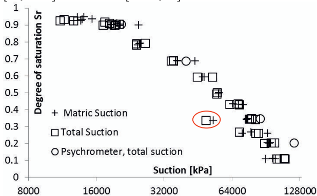
Figure 7. Obtained total and matric suctions for MX-80 bentonite partially saturated with deionised water. Points in the ellipse not taken into account when calculating errors.
