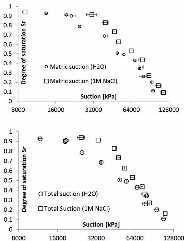
Figure 11. Standard errors (computed based on 3 samples for each average value) for matric and total suction.
