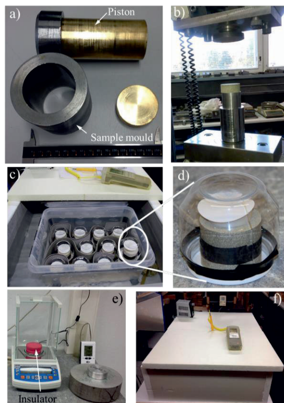
Figure 2. a) tools used for sample pressing, b) compressed specimen being extracted from the sample mould, c) samples kept in the constant-temperature water bath, d) filter paper test assembly, e) insulation placed between the balance and moisture tin, and f) well insulated water bath with temperature control.
