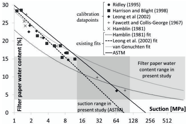
Figure 6. Calibration curves for filter paper and available calibration points matched with approximate range of suctions and filter paper water content in current study. Data courtesy Ms Acikel, after [15-16]. Calibration data points taken from [12,17-19] and fits from [10-12, 14].
