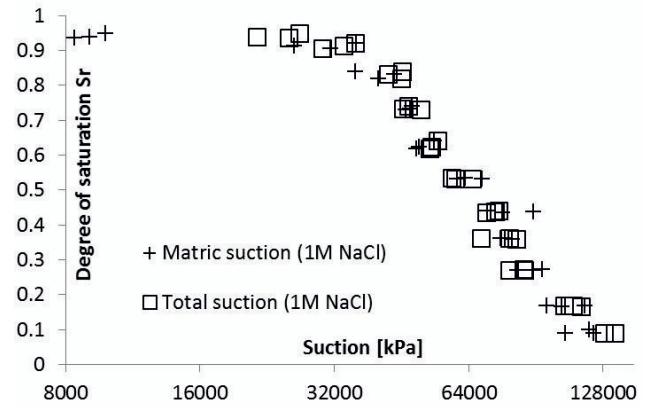
Figure 9. Obtained water retention curve for MX-80 bentonite partially saturated with 1 molar solution of NaCl.
