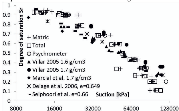
Figure 8. Obtained water retention curve vs literature data on the same material [1, 3, 5-6].
