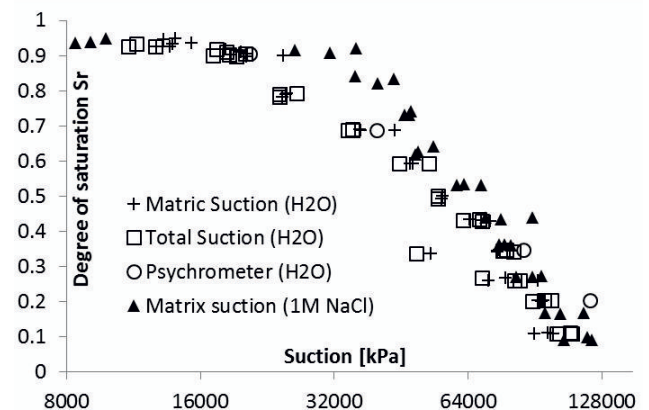
Figure 10. Differences between suctions for samples partially saturated with deionised (H 2 O) and salty water (NaCl)
